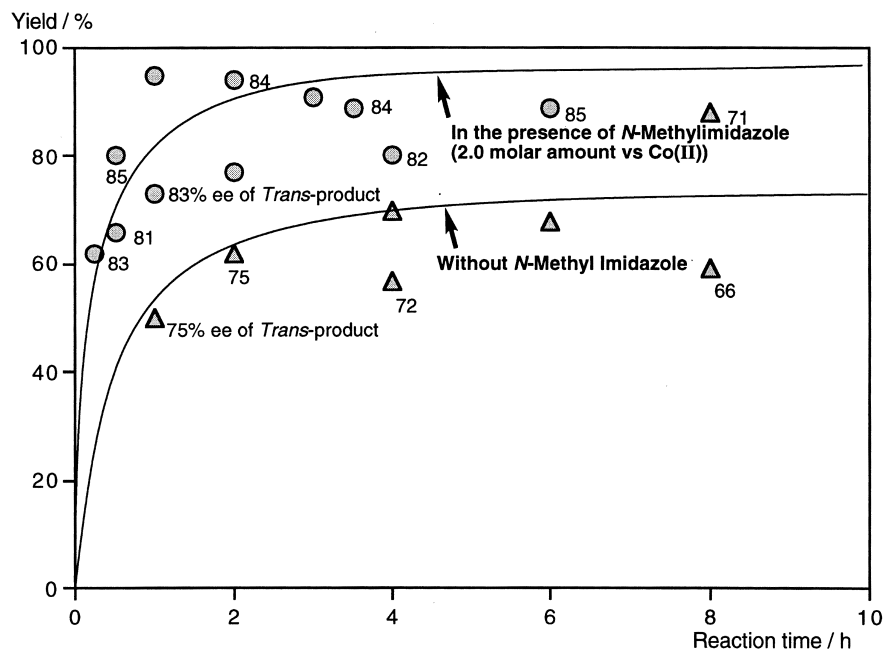
Fig. 1. Time-course of the cyclopropanation reaction in the presence and absence of N -methylimidazole.
