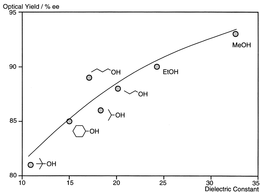
Fig. 3. The dependence of the optical yield of the product on the dielectric constant of the alcohols.
