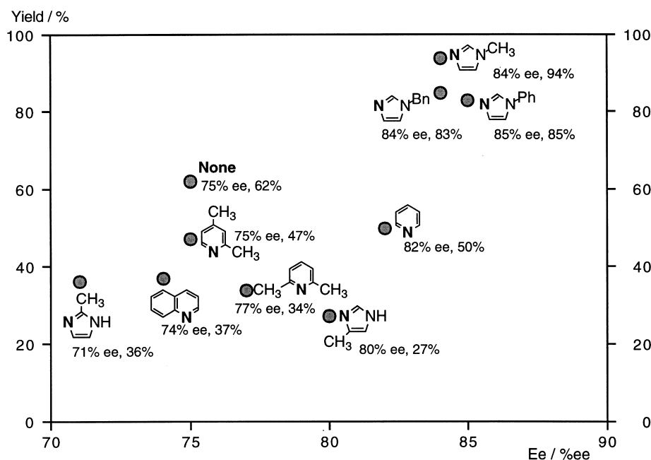
Fig. 2. Relation between yields and enantiomeric excesses for nitrogen-containing heteroaromatics.
